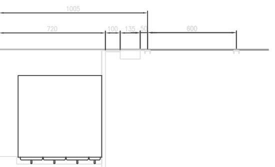
SECTION OF CABINET DESK
